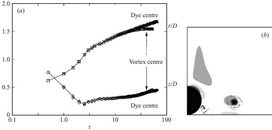
FIGURE 7. (a) Time variation of the axial and radial coordinates of the primary vortex ring obtained from dye particle tracking (outer sets of results) and from following the position of maximum vorticity (inner sets of results). Both sets of results were obtained from numerical simulations. Re = 800 and L/D = 5 . (b) Image showing the differing vorticity and particle centres after a long time, \tau = 60 . Here, the black semicircular area shows the location of the sphere and the grey areas indicate concentrations of vorticity.
