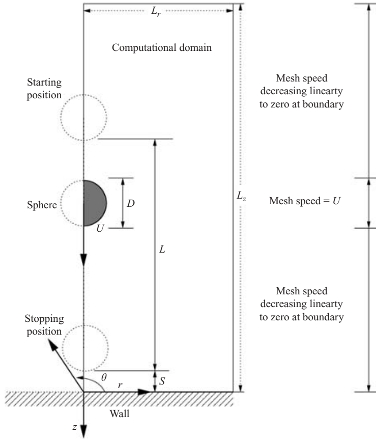
FIGURE 1. Computational setup showing the main parameters. The sphere descends through a running distance L at constant speed U , before stopping at a distance S above the tank floor. The computational domain was specified by domain-size parameters L_z and L_r . Cylindrical polar coordinates were used.
