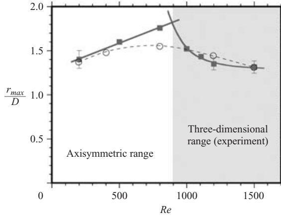
FIGURE 12. Maximum ring radius as a function of Reynolds number. The experimental results are shown by the squares and numerical predictions by the circles. The connecting lines act as a visual aid. The difference between the experimental results and the numerical predictions is due to the different ways of defining the ring position, as discussed in the text, and the fact that the flow is three-dimensional for Re > 1000 in the experiments.
