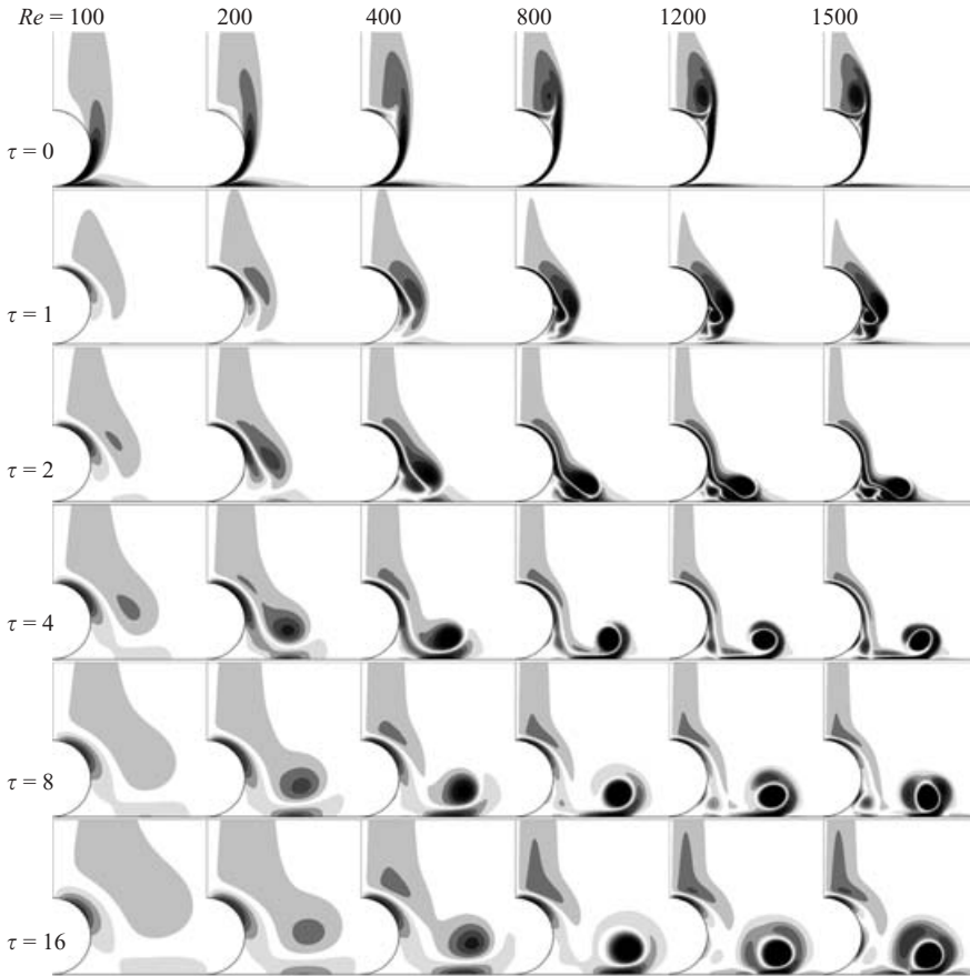
FIGURE 10. Vorticity contours showing the evolution of vortex structures from formation, threading over the sphere and impact with the wall. Contours are shown for Re = 100, 200, 400, 800, 1200 and 1500 . At larger times the contour ranges are reduced for better depiction of the vorticity-field structure. However, for each time value the contour levels are the same.
