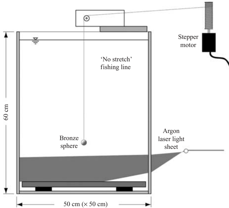
FIGURE 3. Experimental setup showing the main features. Details are provided in the main text.
