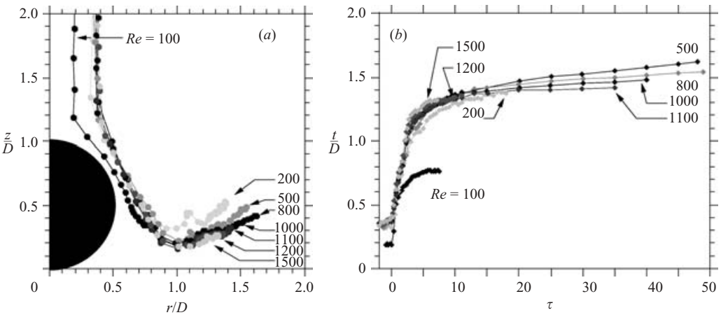
FIGURE 8. Effect of Reynolds number, as observed by experimental dye visualizations: (a) the trajectories of the primary vortex ring; (b) the radial position of the primary ring as a function of time.
