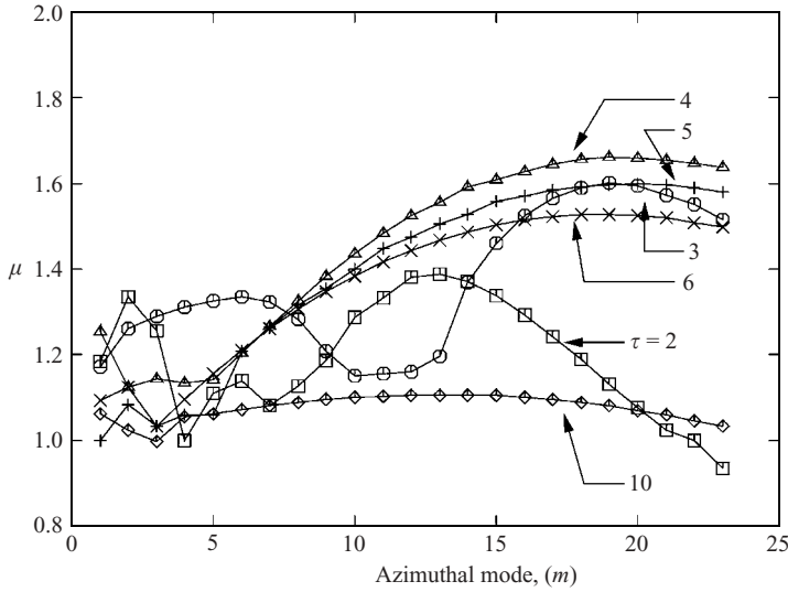
FIGURE 21. Amplification factor per unit time, \mu , associated with the frozen axisymmetric base flow as a function of azimuthal mode number and non-dimensional time. Here Re = 1200 and L/D = 5 . The various curves are for the \tau -value shown.
