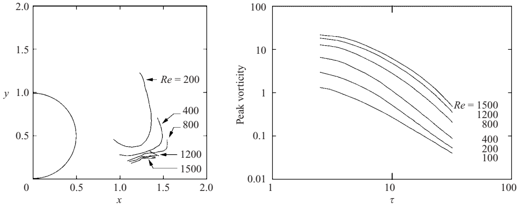
FIGURE 9. (a) Trajectories of the vorticity maximum of the primary vortex ring after impact ( 2.5 < \tau < 52 ) obtained from axisymmetric numerical simulations. Paths corresponding to different Reynolds numbers are marked. (b) Post-impact evolution of the primary-ring peak vorticity as a function of Reynolds number.
