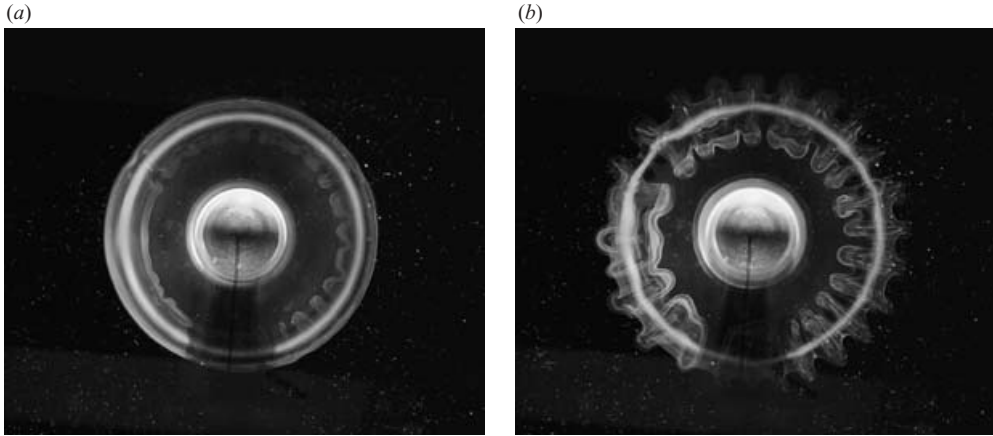
FIGURE 19. Dye visualization showing the three-dimensional structure of the vortical ring system for Re = 1500 and L/D = 5 . (a) \tau = 4 , (b) \tau = 9 .
