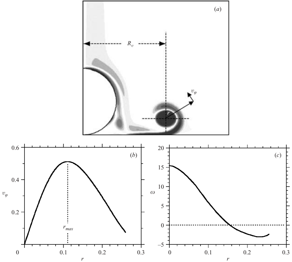
FIGURE 25. Analysis of the flow field for Re=1200 and L/D=5 at \tau=4 . (a) azimuthal vorticity distribution. Profiles of (b) circumferential velocity and (c) vorticity of the primary vortex, averaged over \varphi .
