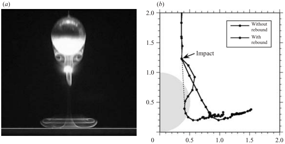
FIGURE 18. (a) Experimental dye visualization of the flow at \tau = 2 after sphere impact with rebound. Re = 800 , L/D = 5 . (b) Trajectory of the primary vortex with and without rebound for the same parameters.
