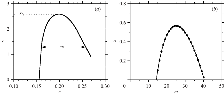
FIGURE 26. (a) Local inviscid growth rate s = (-\Phi)^{1/2} and (b) global viscous growth rate as functions of the azimuthal wave number m , for the flow field in figures 25b and 25c, according to (4.4).
