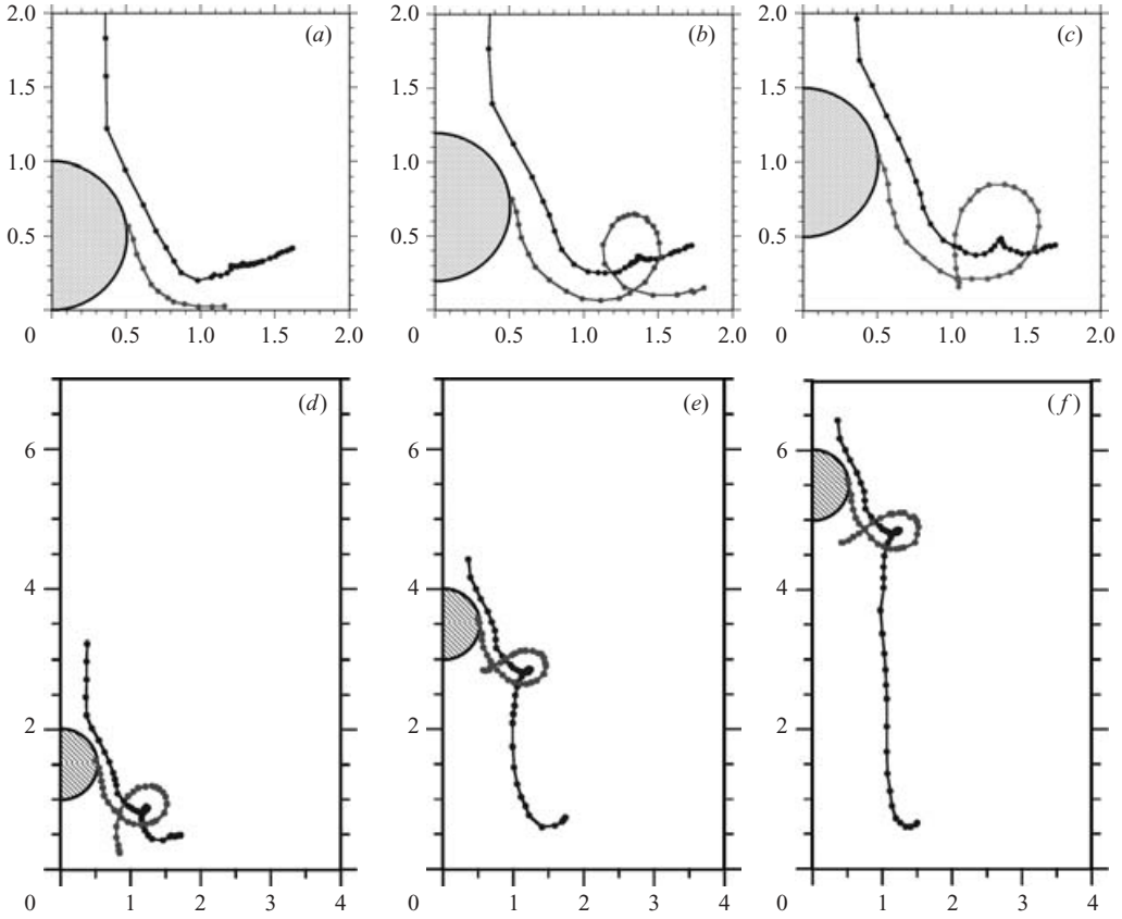
FIGURE 17. Trajectories of the primary (black line) and secondary (grey line) structures at Re=800 and L/D=5 , for different stopping distances. (a) S/D=0 , (b) S/D=0.2 , (c) S/D=0.5 , (d) S/D=1 , (e) S/D=3 , (f) S/D=5 .
