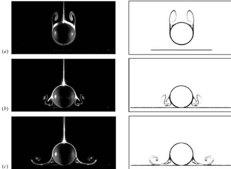
FIGURE 4. Experimental dye visualizations and numerical particle tracers, both initially located at the sphere surface. Re = 500 , L/D = 5 , S/D = 0 . Relative to the time of impact, the times shown are (a) \tau = -0.25 , (b) \tau = 1.50 and (c) \tau = 3.80 .
