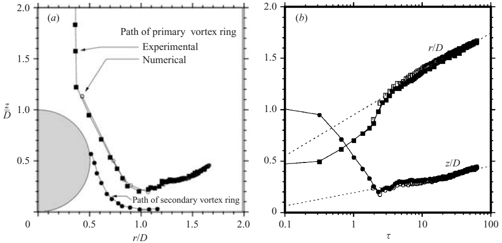
FIGURE 6. (a) Trajectories of the primary and secondary vortex rings as given by the centroid of the dye spiral (experiments) or the centroid of the tracer particles (numerical simulations). (b) Variation in radial and axial coordinates of the primary ring with time, also showing asymptotic projections. Re = 800 , L/D = 5 .
