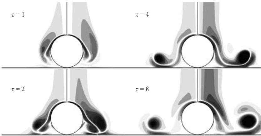
FIGURE 16. Development of the vorticity field for different running distances and for Re = 500 , obtained from numerical simulations. For each figure, the left- and right-hand parts depict the vorticity field for L/D = 5 and 25 respectively. Note that the vorticity contour levels are the same for all images.
