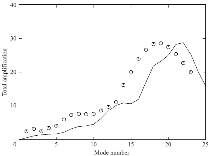
FIGURE 22. Amplification factor of azimuthal perturbations as function of mode number for the period 2 < \tau < 10 . The symbols indicate the total amplification factor calculated by temporally integrating the quasi-steady amplification rates from the previous figure. The line gives the growth of each mode number obtained directly from a DNS calculation.
