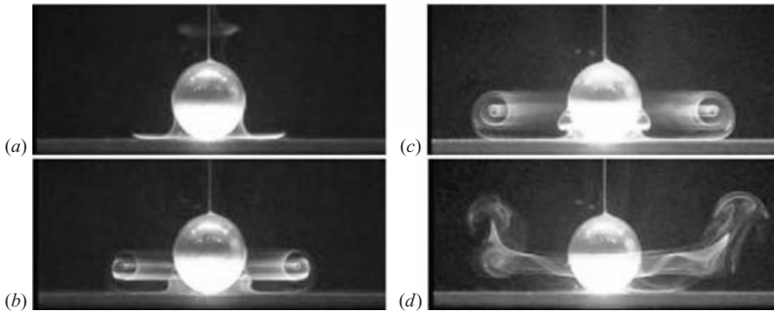
FIGURE 14. Experimental dye visualizations of the flow for Re = 800 at \tau = 25 for different running distances. The images correspond to (a) L/D = 1 , (b) L/D = 2 , (c) L/D = 5 and (d) L/D = 10 .
