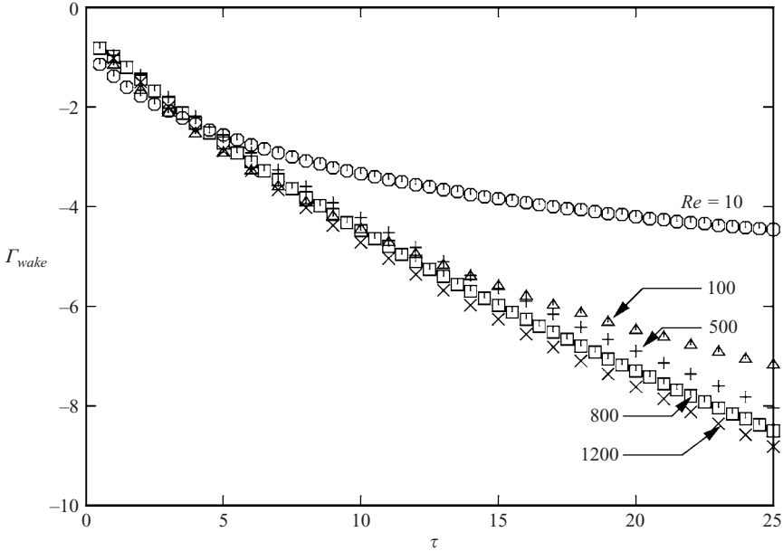
FIGURE 15. Circulation contained in the axisymmetric wake from a sphere started impulsively from rest as a function of time, for different Reynolds numbers.
