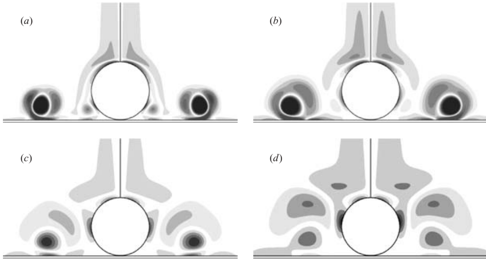
FIGURE 11. Vorticity contours showing the long-time-evolution vortex structures for Re = 1500 . (a) \tau = 8 , (b) \tau = 16 , (c) \tau = 32 , (d) \tau = 52 . For each image the contour levels have been adjusted to show all the vortex structures present. Note the net movement of the primary vortex ring back towards the axis.
