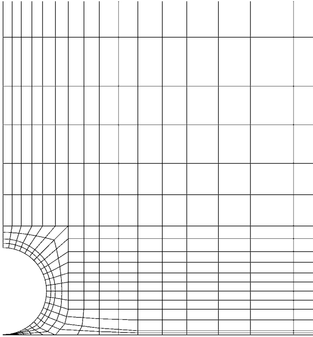
FIGURE 2. Close-up of the mesh in the neighbourhood of the sphere at the point of impact. Only macro-elements are shown. Within each macro-element, the mesh is subdivided into n_x \times n_y nodes. Typically, n_x = n_y = 5 – 10 , depending on the Reynolds number.
